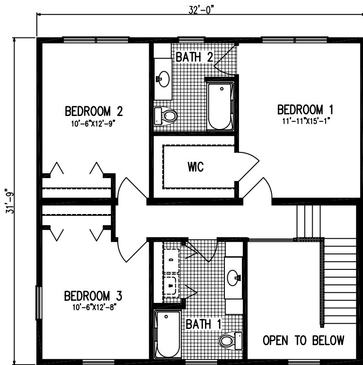
2ND FLOOR- 1024 SQ FT
