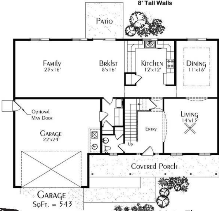
MAIN FLOOR SqFt. = 1399 9' Tall Walls
