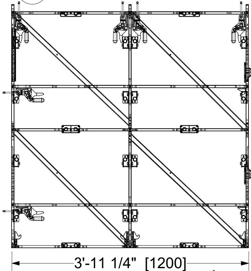
1 Front View 1" = 1'0"
