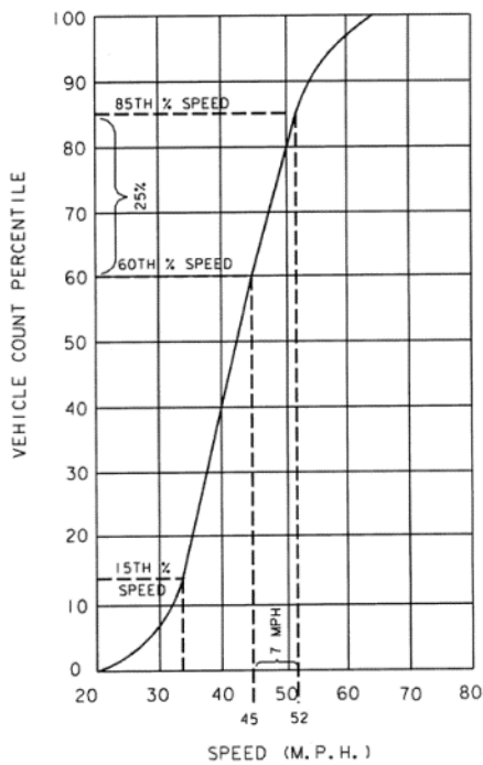
Figure 3-1. Cumulative speed distribution curve
