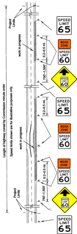
Figure 2-3. Typical construction speed zone.
