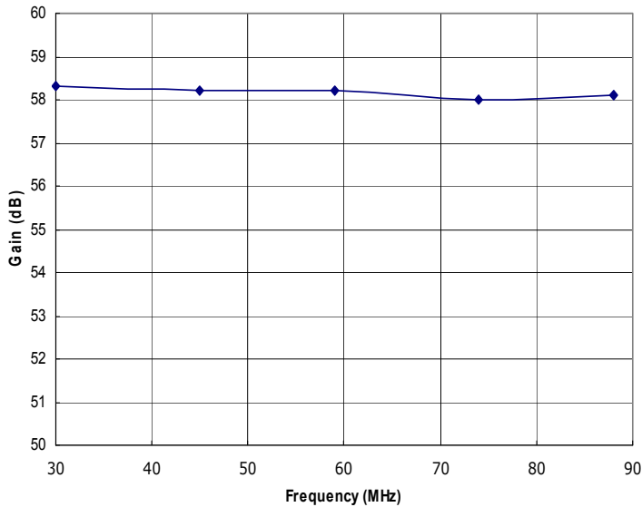
Figure 1: RFM30-88-350-HSD Typical Gain @ P out = 350W.
