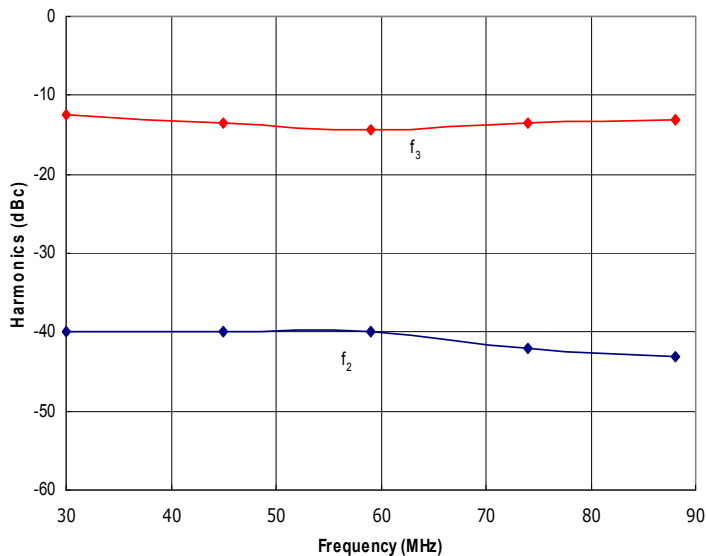
Figure 3: RFM30-88-350-HSD Typical f 2 and f 3 @ P out = 350W.
