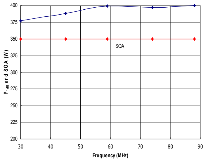
Figure 4: RFM30-88-350-HSD Typical P 1dB and Safe Operating Area (SOA). The amplifier is capable of delivering more power than it is safe to generate. Do not exceed the SOA shown above without first contacting RFMPT to discuss your application.
