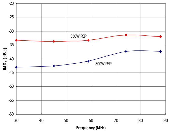
Figure 2: RFM30-88-350-HSD Typical IMD 3 @ 350W and 300W PEP, Δf = 100kHz.
