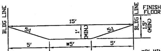
TYPICAL SWALE SECTION
