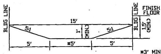
TYPICAL SWALE SECTION
