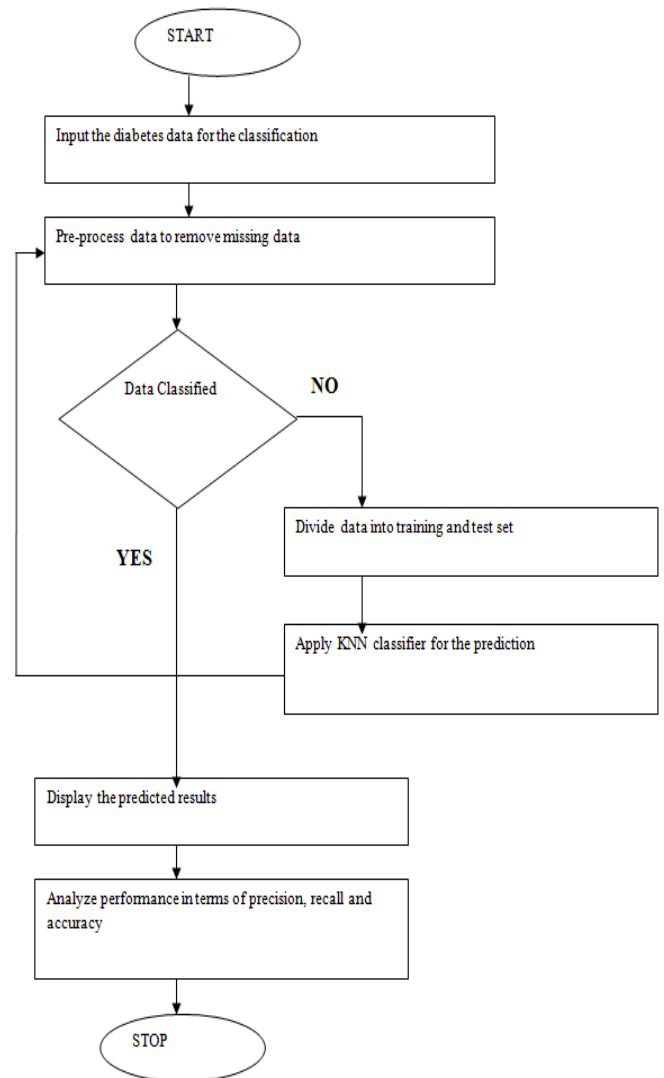
Fig.1: Proposed Methodology
