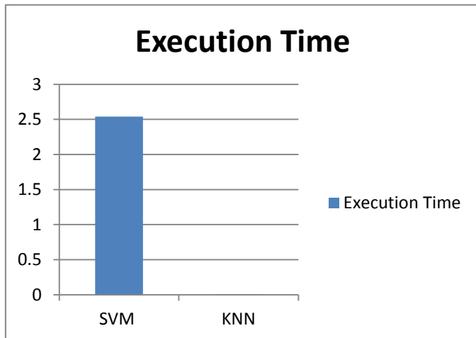
Fig.3: Execution Time
