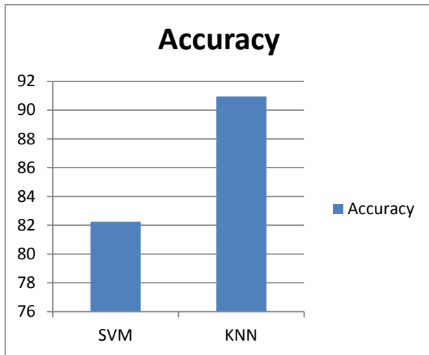
Fig.2: Accuracy Comparison
