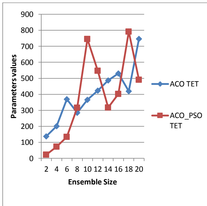
Figure 4.1: Comparison graph of TET of ACO and ACO_PSO using GENOME:
