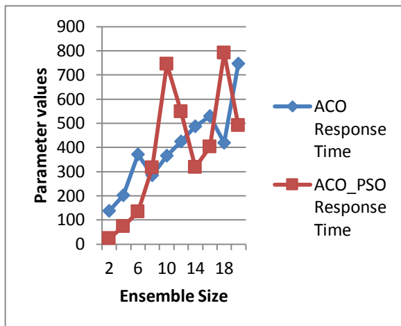
Figure 4.3: Comparison graph of Response time of ACO and ACO_PSO using GENOME:
