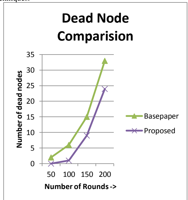
Fig 3: Number of dead Node Comparison
