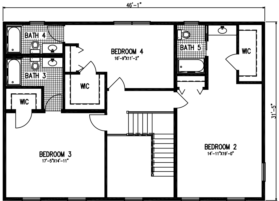
2ND FLOOR- 1472 SQ FT
