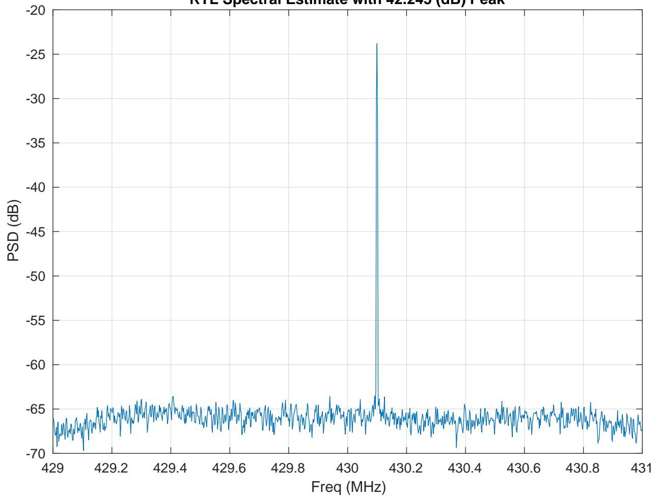
RTL Spectral Estimate with 42.245 (dB) Peak
