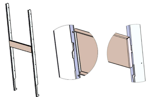
Shown Illustration: CAD view of patented-designed concealed fastening rail system, wall panel back view, wall panel front view)
