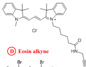
(C) Cy3 alkyne
