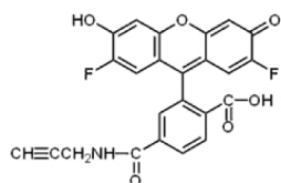
(C) Cy3 alkyne
