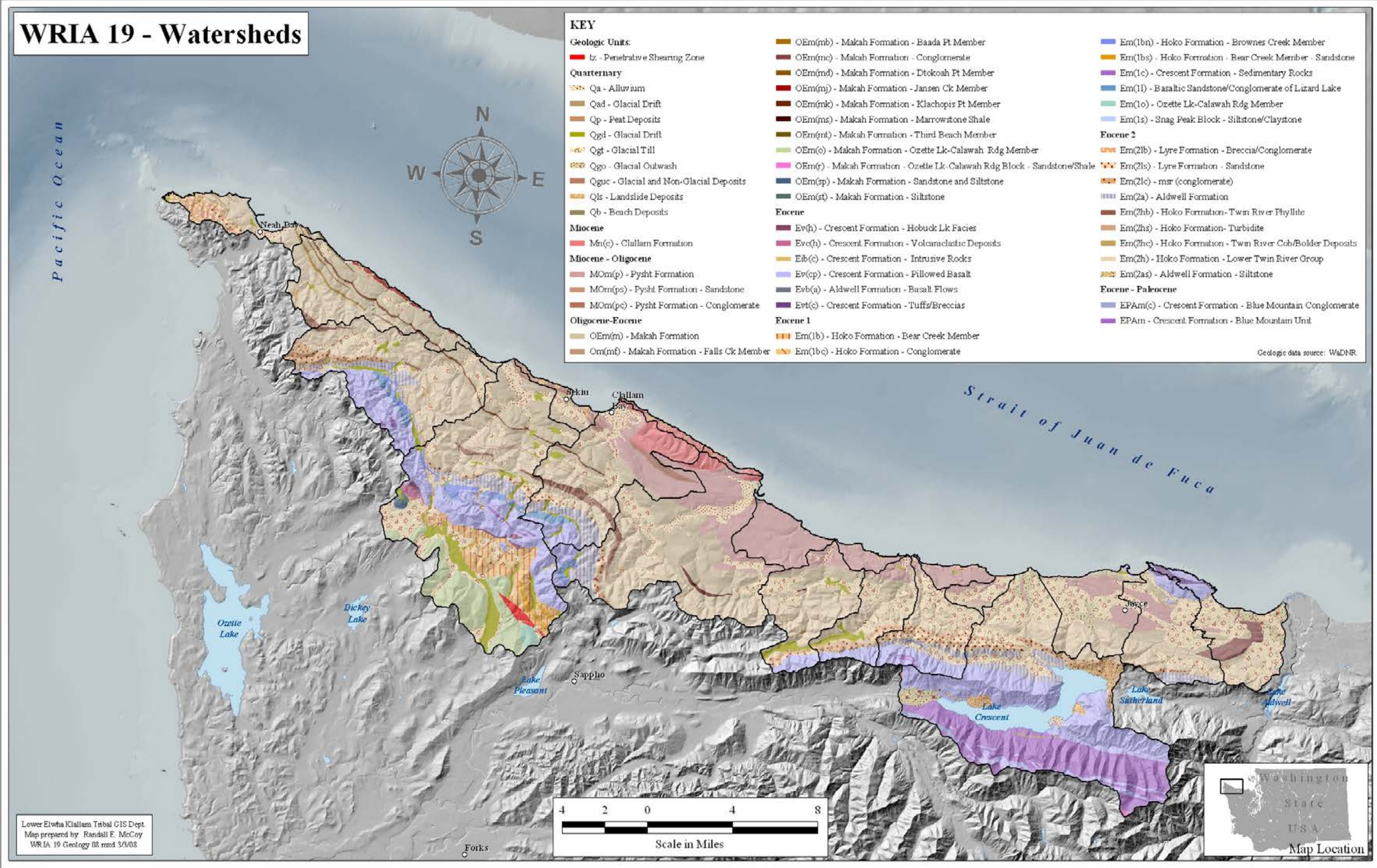
Figure 2. Geologic map of the WRIA 19 watershed (source: WDNR geologic data from Schasse 2003).
