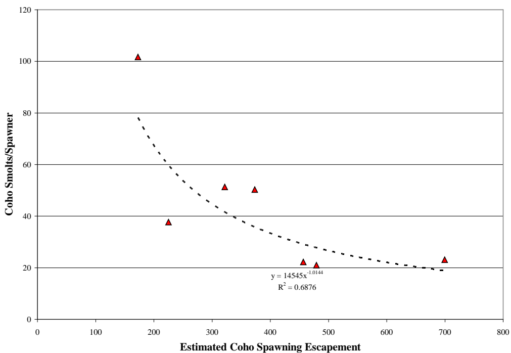
Figure 40. Deep Creek coho smolts produced per spawner versus coho spawning escapement.
