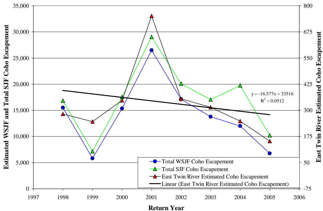
Figure 27. Estimated coho spawning escapement for SJF, WSJF, and East Twin River for return years 1998-2005 (source: WDFW and Lower Elwha Tribe, unpublished data).
