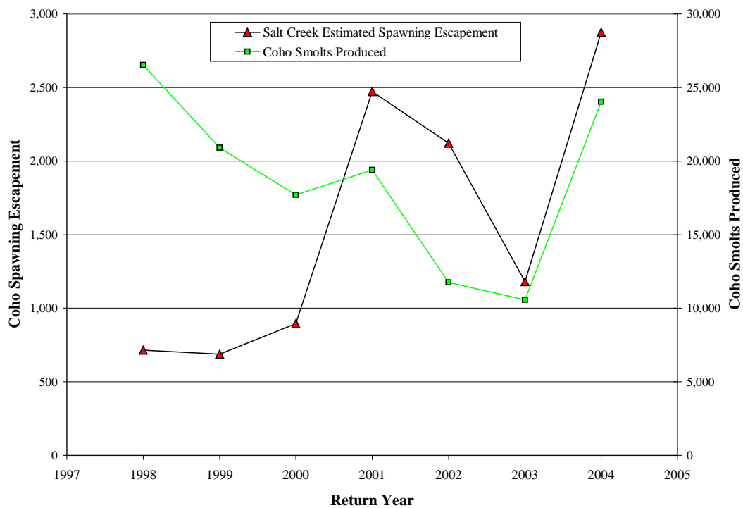
Figure 20. Salt Creek coho spawning escapement and subsequent number of smolts produced (source: Lower Elwha Tribe, unpublished data).
