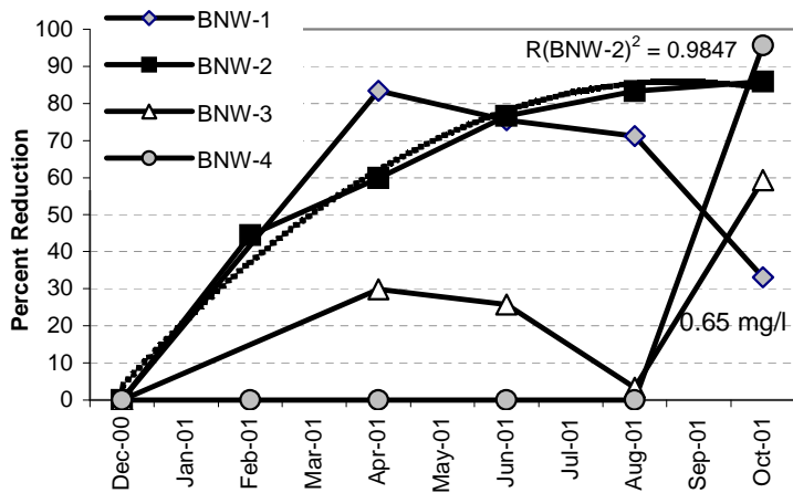
FIGURE 5. Percent reduction of MTBE in BioNets.
