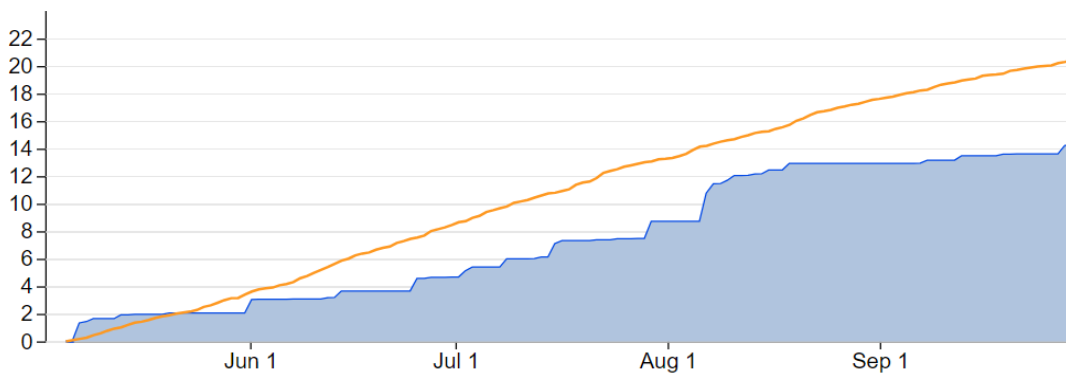
Accumulated Precipitation
