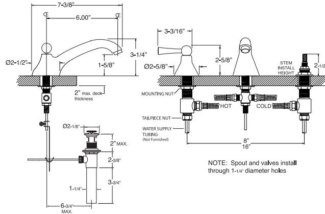
Widespread Lav Faucet
