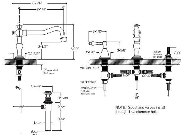
Widespread Lav Faucet
