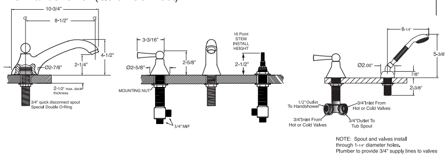
Roman Tub Set w/ Diverter & Handshower (Quick Connect)
