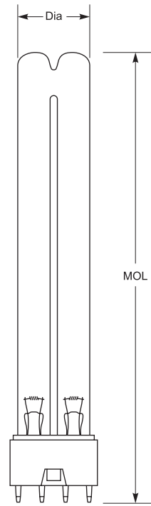
2G11 Base
