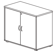
EXD 880 SWINGING DOOR CABINET 804W x 402D x 848H
