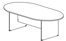
OVAL CONFERENCE TABLE EXO 18 1800W x 900D x 745H EXO 24 2400W x 1200D x 745H
