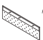
18 HG/WR HALF GLASS DESKING PANEL 1800W x 450H x 18D 1800W x 600H x 18D 1500W x 450H x 18D 1500W x 600H x 18D 1200W x 450H x 18D 1200W x 600H x 18D
