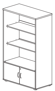
EXB 741 BOOK SHELF 804W x 402D x 1670H
