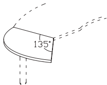
SIDE CONNECTION TR700 1300W x 700D x T25 TR800 1500W x 800D x T25
