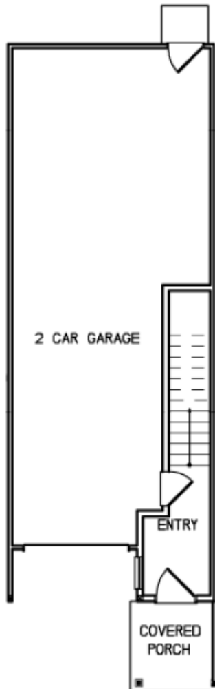
1st Floor
