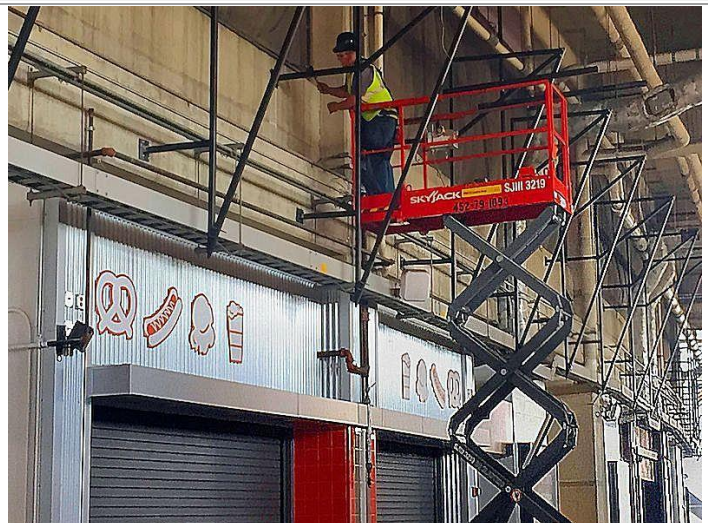
The stretching frame was installed on an existing steel frame...
