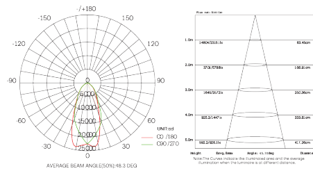
50° Beam Angle 200W
