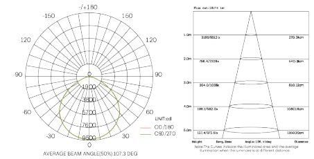
110° Beam Angle 200W
