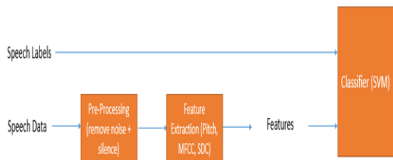
Fig.1: Age and Gender Recognition System Training
