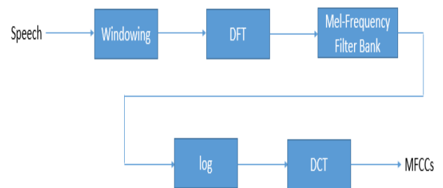
Fig.5: Steps for MFCC Computation
