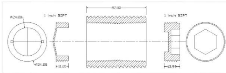
1 inch Check Valve, Plug & Pipe Wall Insert
