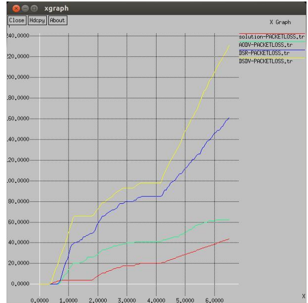
Fig 2: Packetloss Comparison
