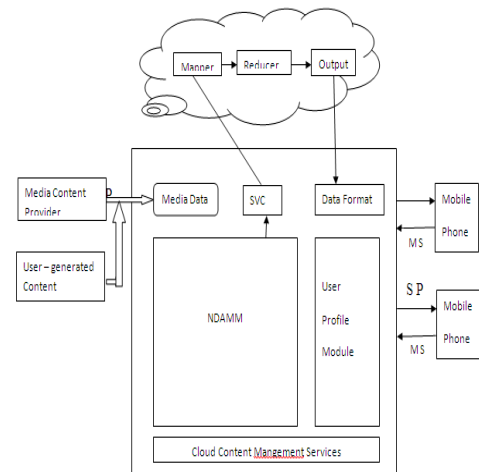
Fig: Architecture
