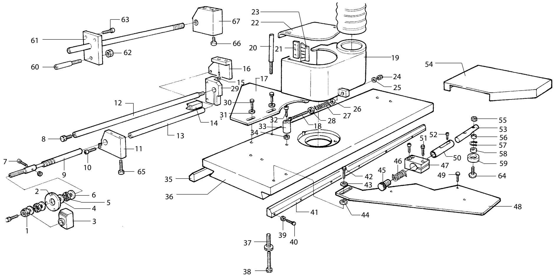
VERTICALE SINISTRO LEFT VERTICAL SPINDLE
