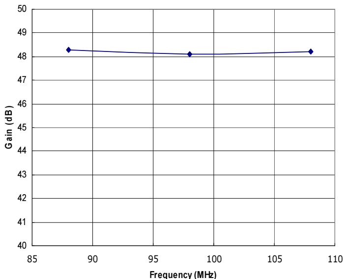
Figure 1: RFPS88-108-25 Typical Gain @ P out = 25W.
