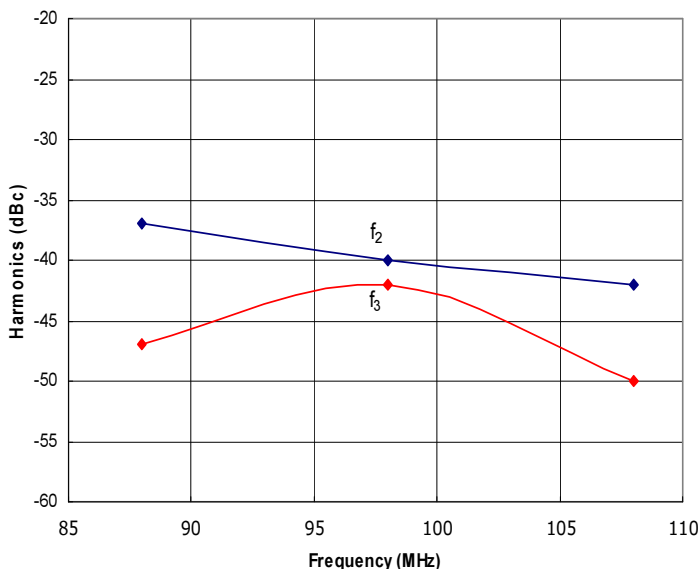
Figure 3: RFPS88-108-25 Typical f 2 and f 3 @ P out = 25W.
