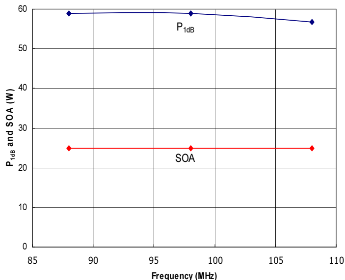
Figure 4: RFPS88-108-25 Typical P 1dB and Safe Operating Area (SOA). The amplifier is capable of delivering much more power than it is safe to generate. Do not exceed the indicated SOA.
