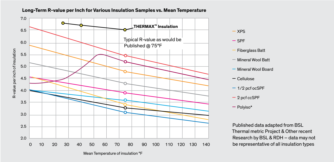
Figure 3: Common Representation of Selected Insulation R-Values as a function of Mean Temperature with THERMAX Brand Insulation properties added.
