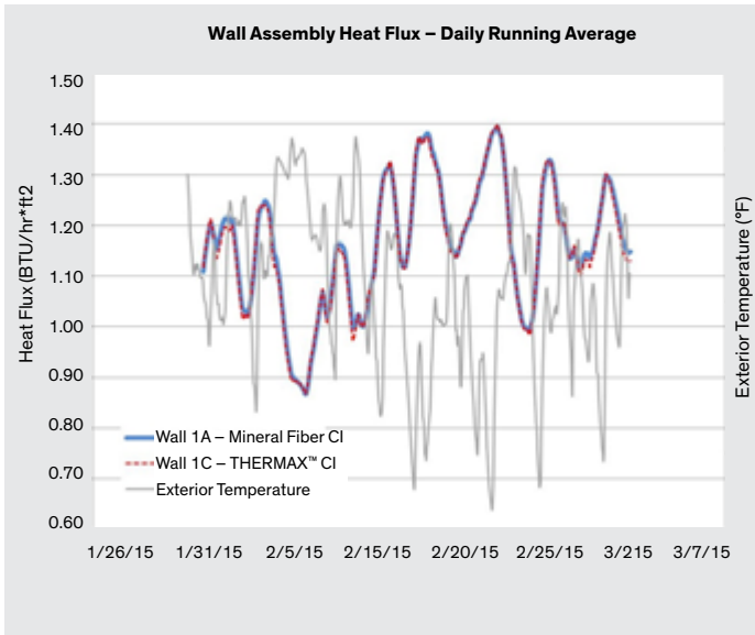
Figure 4: Real World Heat Flux through Two Wall systems (Both R10 CI) in Midland, Michigan during February, 2015.
