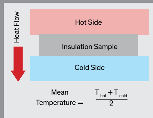
Figure 6: Basic set up for measuring heat flow and the resulting R-Value for an insulation material.
