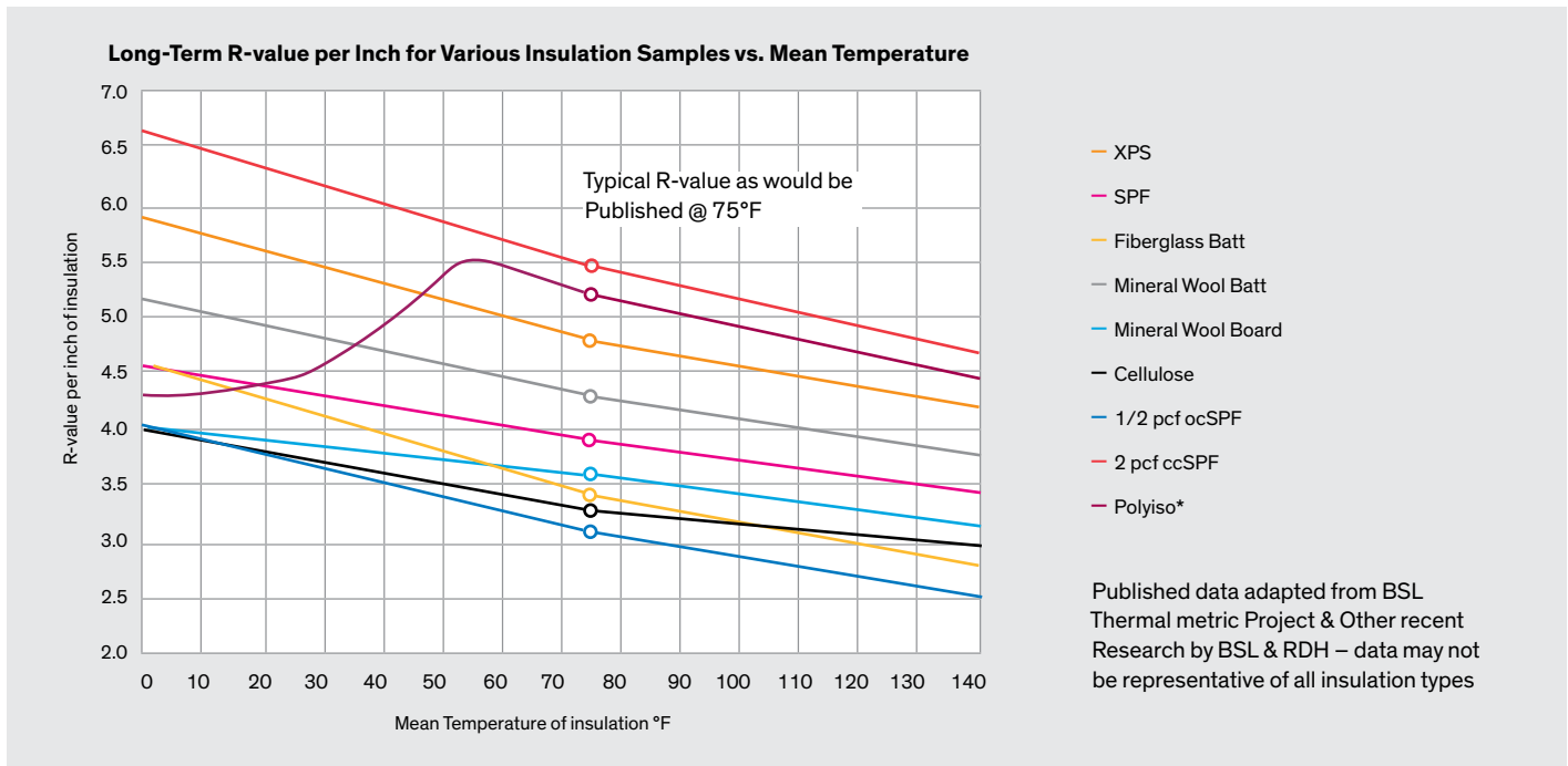
Figure 2: Common representation of selected insulation R-Values as a function of Mean Temperature
