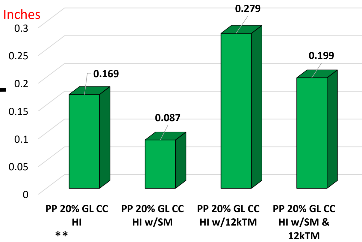
Injection Molding ICP 5" Test Panels Warp Study
