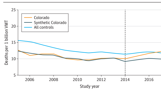
Figure 1. Traffic Fatalities per 1 Billion Vehicle Miles Traveled (VMT), Colorado vs Synthetic Colorado
