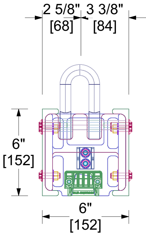
3 Right View 3"=1'0"
