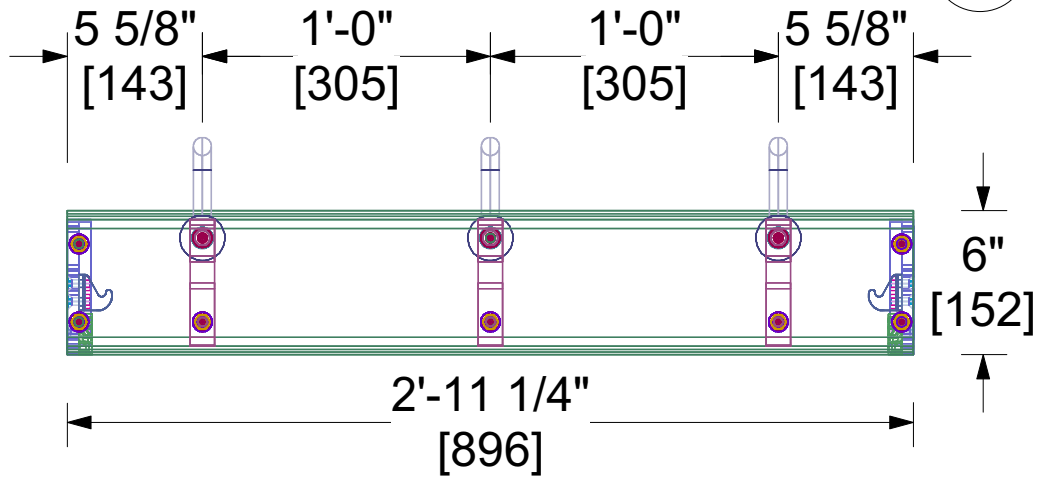
1 Front View 1-1/2"= 1'0"
