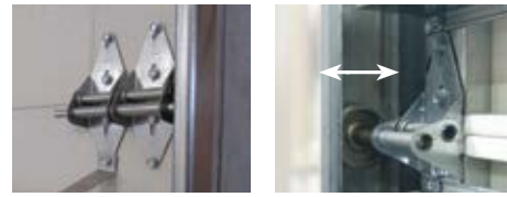
Double-end hinge
