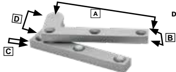
Fixed Pin Pivot Hinge
