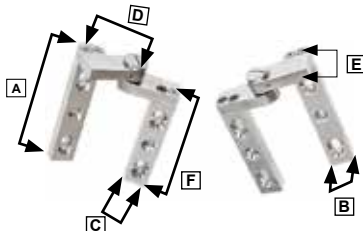
Removable Pin Intermediate Pivot Hinge
