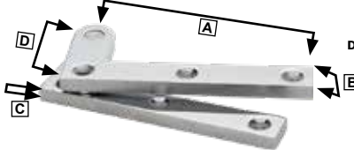
Removable Small Form Pin Pivot Hinge
