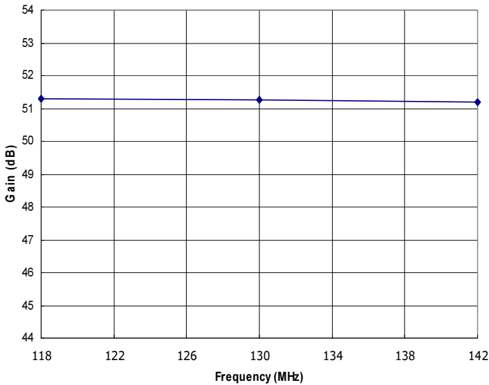
Figure 1: RFM118-142-50-HSD Typical Gain @ P out =50W.
