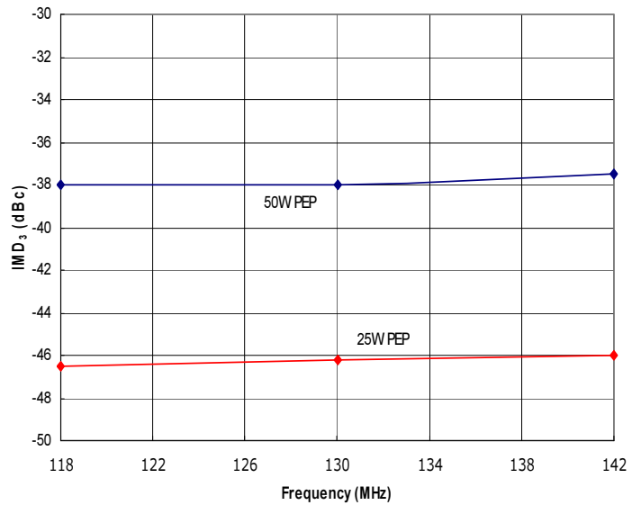
Figure 2: RFM118-142-50-HSD Typical IMD 3 @ 50W and 25W PEP, Δf=10kHz and Δf=100kHz.
