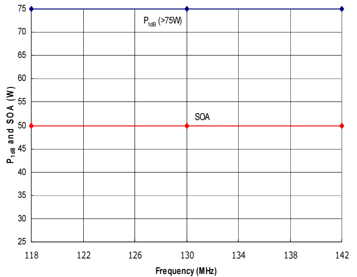
Figure 4: RFM118-142-50-HSD Typical P 1dB and Safe Operating Area (SOA). The amplifier is capable of delivering much more power than it is safe to generate. Do not exceed the SOA shown above without first contacting RFMPT to discuss your application.
