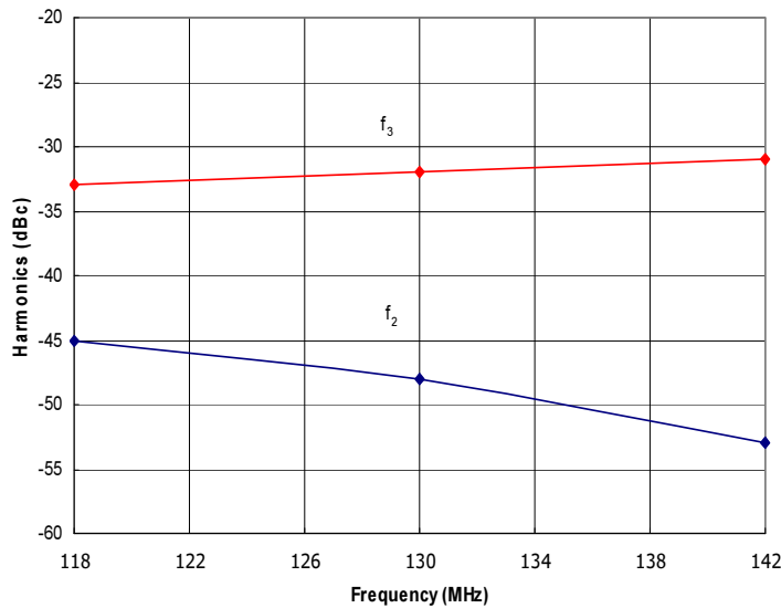
Figure 3: RFM118-142-50-HSD Typical f 2 and f 3 @ P out =50W.
