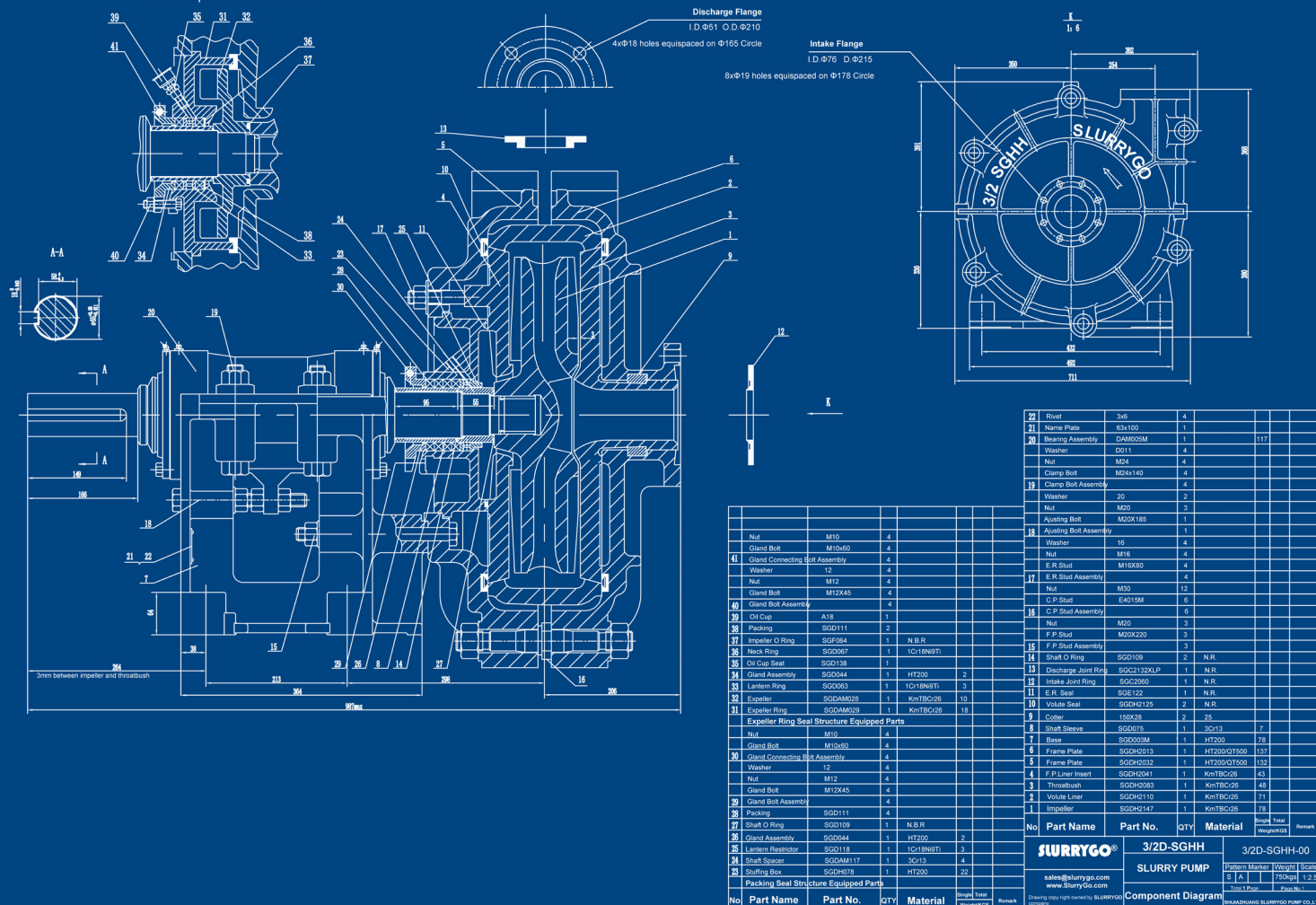
Metal Expeller Seal Structure
