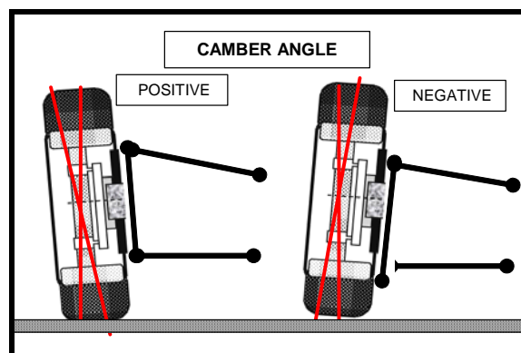
Figure 54 - Camber
