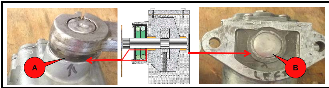
Figure 25 – Leak Points
