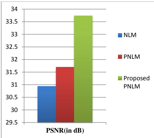
Figure 2: PSNR Comparison
