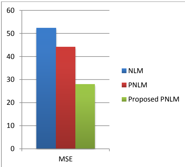
Figure 3: MSE Comparisons
