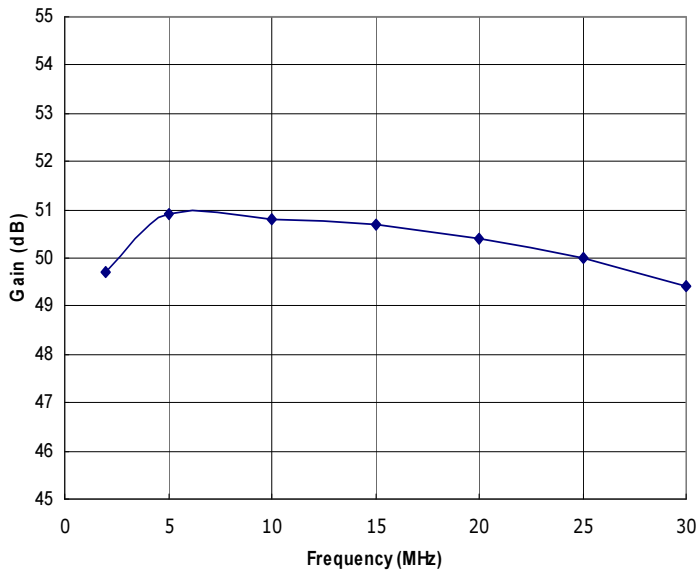
Figure 1: RFPS2-30-50 Typical Gain @ P out = 50W.
