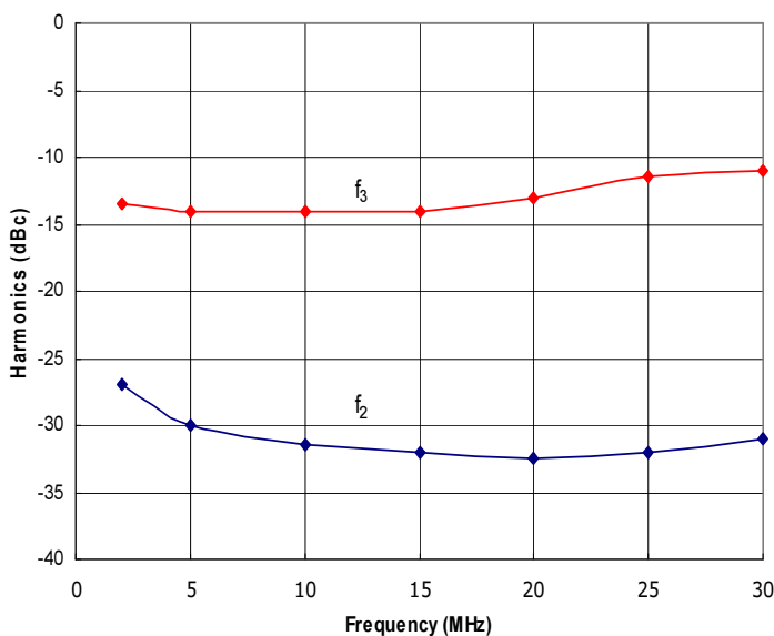
Figure 3: RFPS2-30-50 Typical f 2 and f 3 @ P out = 50W.
