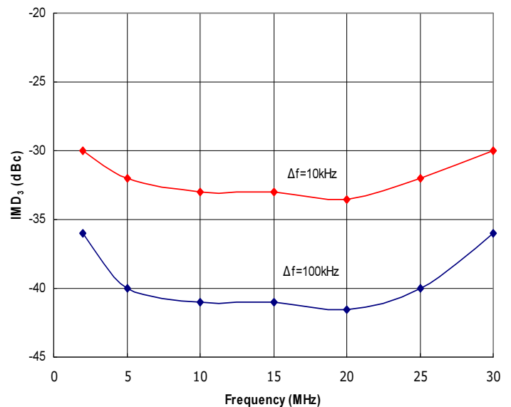
Figure 2: RFPS2-30-50 Typical IMD 3 @ 50W PEP, Δf=10kHz and Δf=100kHz. For improved linearity, see our RFPS2-30-25 Class A amp.
