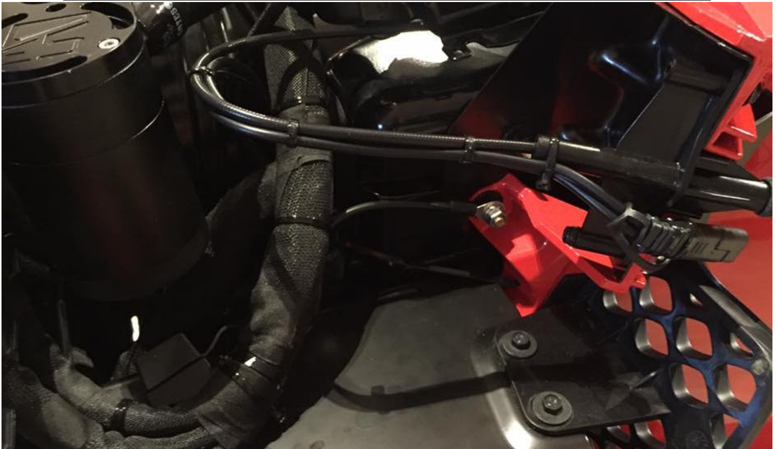
Additional View Of Recommended Wiring Layout
