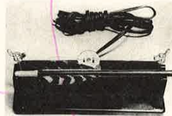
BHB4—Black Hawk Feather Burner. A burner designed for the home draftsman and for home repairs. Completely safe. Does not have transformer. In place of transformer, plug in an electric iron or other appliance in plug shown in base. This will reduce current to the burning wire. Will not work unless appliance is plugged in receptacle. Partially assembled with complete instruction sheet.
