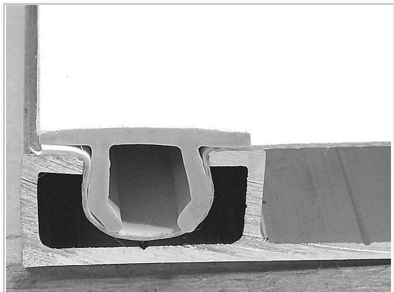
Details of the TS23 aluminum extrusion and the TS79W (White PVC Insert) stretching a printed vinyl.
