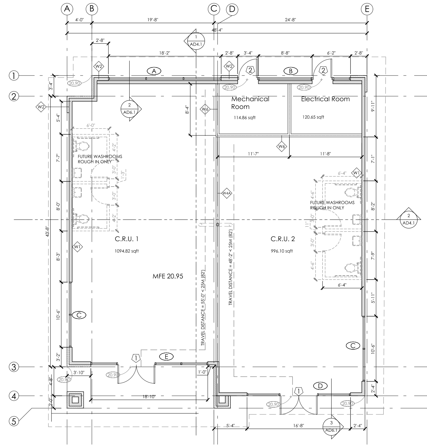
1 Building D (East)- Floor Plan AD2.1 Scale: 3/16" - 1'
