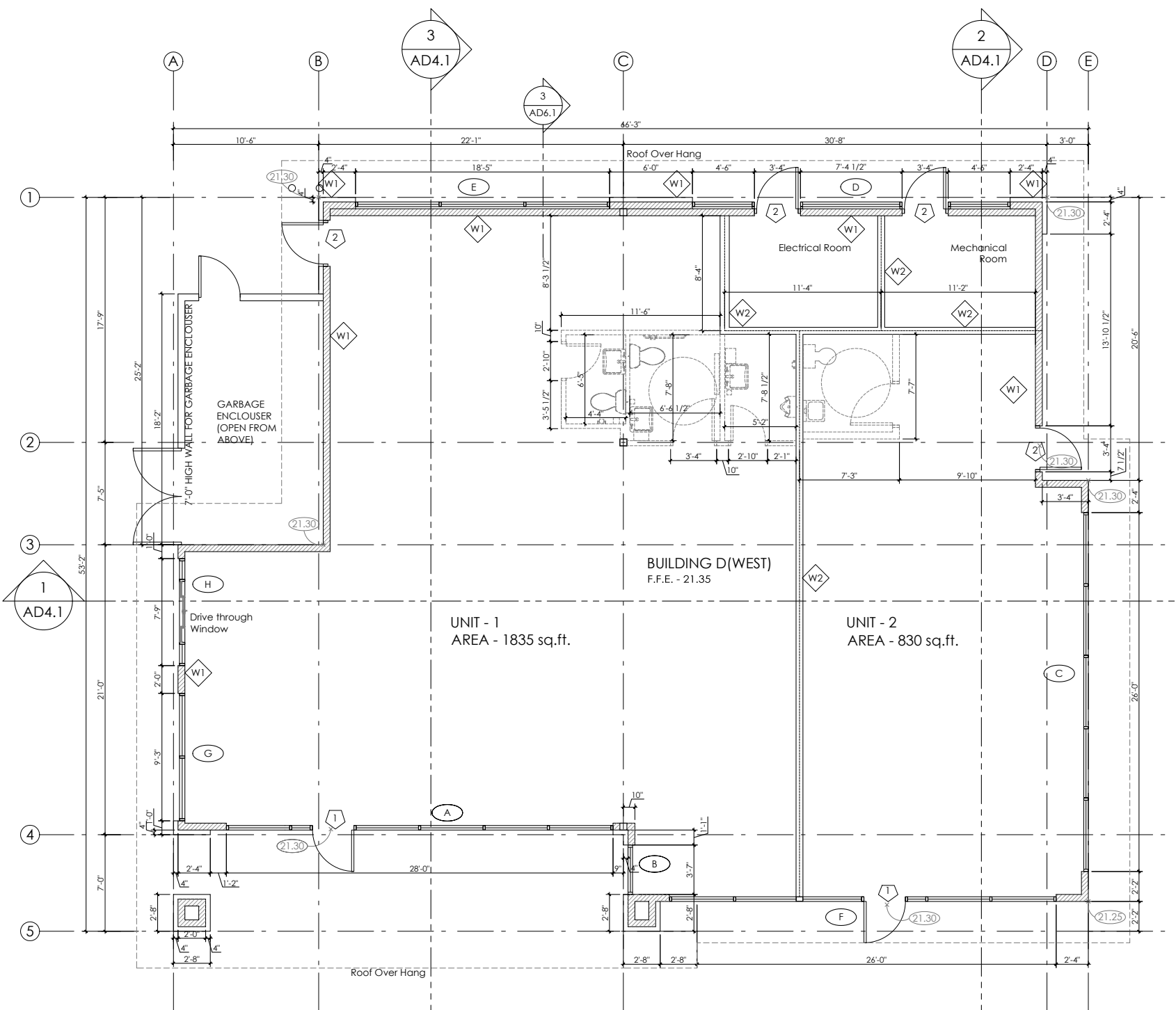
1 Building D (West)- Floor Plan AD2.1 Scale: 1'-3/16"
