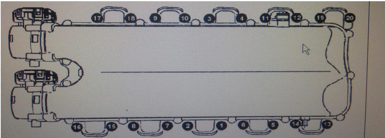
Recommended Tightening Pattern (Per 2008 Service Manual)
