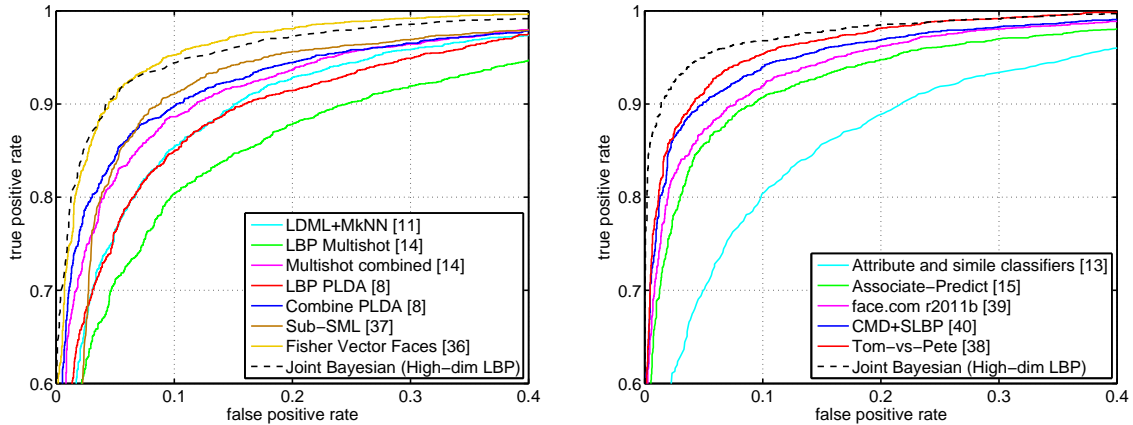
Fig. 4: Comparison with state-of-the-art methods on LFW. Without outside training data(left) and with outside training data(right). Note that Joint Bayesian automatically determines the subspace dimension and here we artificially truncate singular values to produce lower-dimensional models merely for purposes of comparison.
