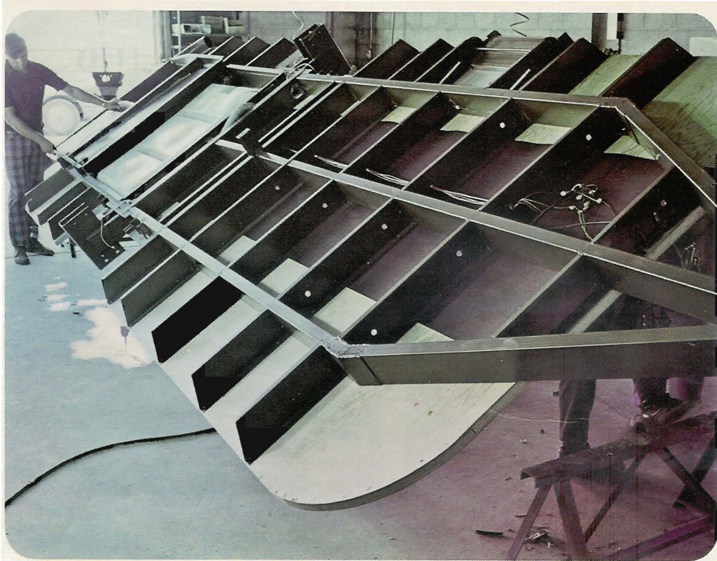
Triple-beam frame of heavy-duty steel is first step in sturdy, tight construction for every road and weather condition.
