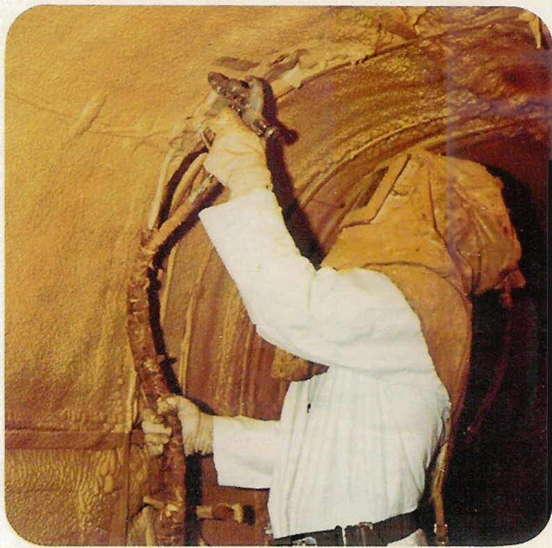
Thermo-X urethane foam is sprayed on throughout interior. It hardens permanently in place to seal out heat, cold, dust and noise while reinforcing walls and roof.
