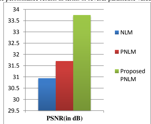
Fig.2: PSNR Comparison
