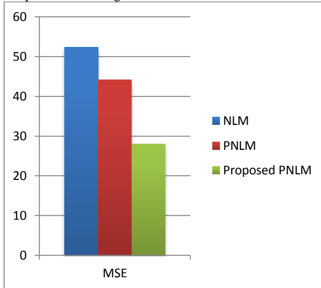
Fig.3: MSE Comparisons
