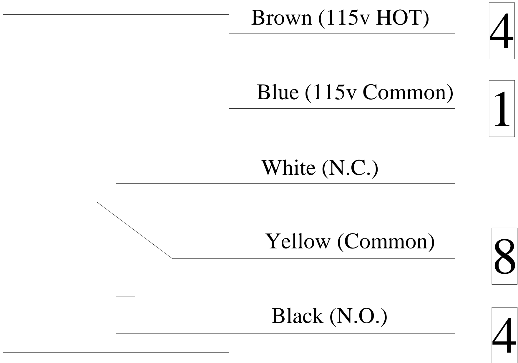
Q45VR3 Photo Sensor Wiring
