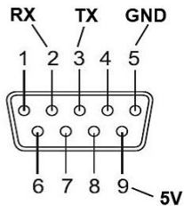
DB9 Male Connector (on available serial Harness)
