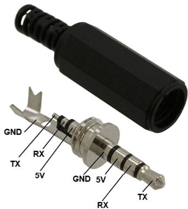
3.5 mm Stereo Jack (4 connections)
