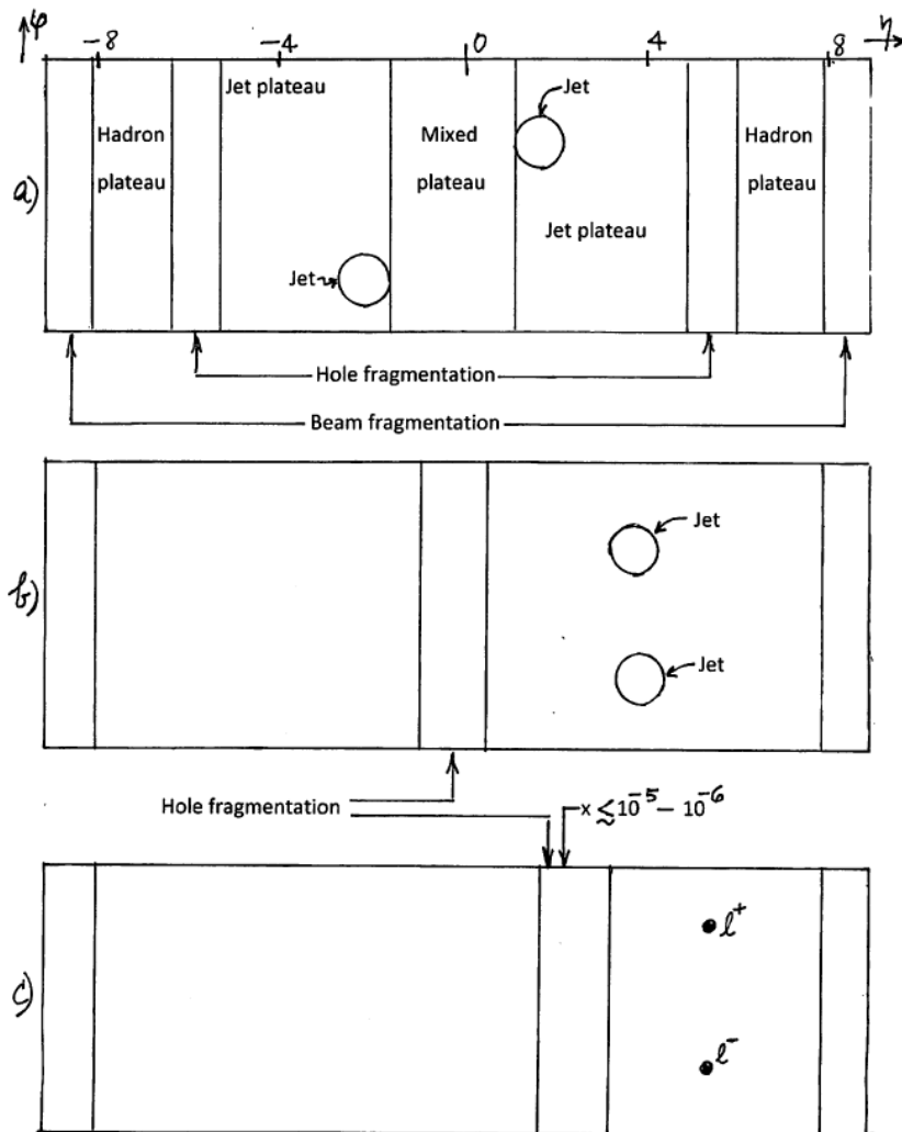
Fig. 4. Lego plots at the LHC energy scale for (a) a typical dijet event, for (b) a boosted dijet event appropriate for the detailed study of hole fragmentation, and for (c) probing parton distributions via the Drell-Yan process at values of x < 10^{-5} - 10^{-6} .
